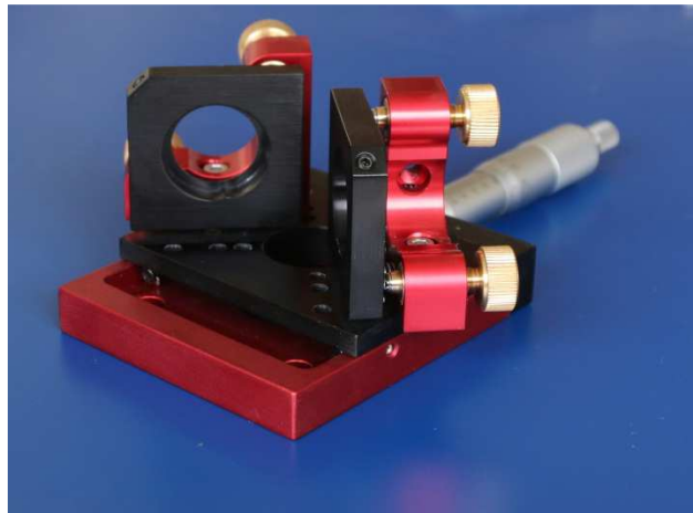
Variable Delay-Line with 2 mirror mounts
