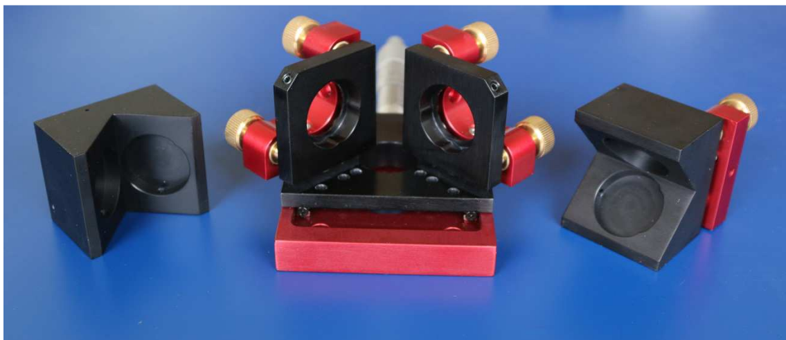
Variable Delay-Line with 2 mirror mounts, one constant 360° circle reverse control and one 360° circle reverse control with mirror mount, also motorized with PiezoMike
